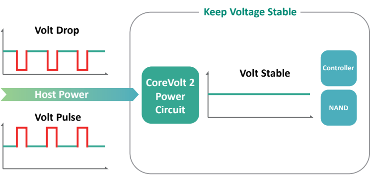
Figure 1: CoreVolt 2 – Power Stabilization Mechanism
